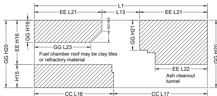
Section G-G
